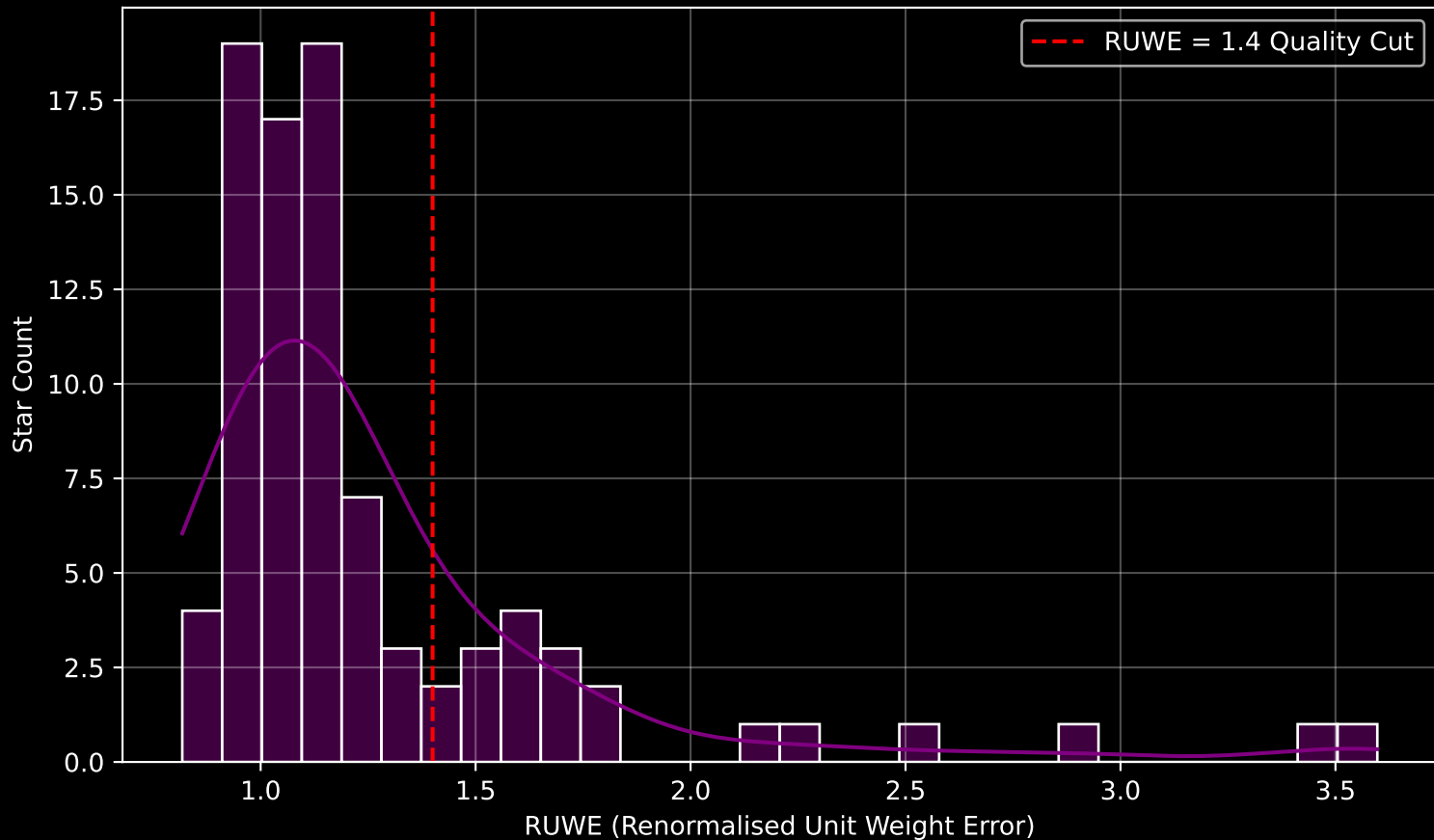
GALAH DR4 Field [6683] RUWE Distribution (n= 89)
