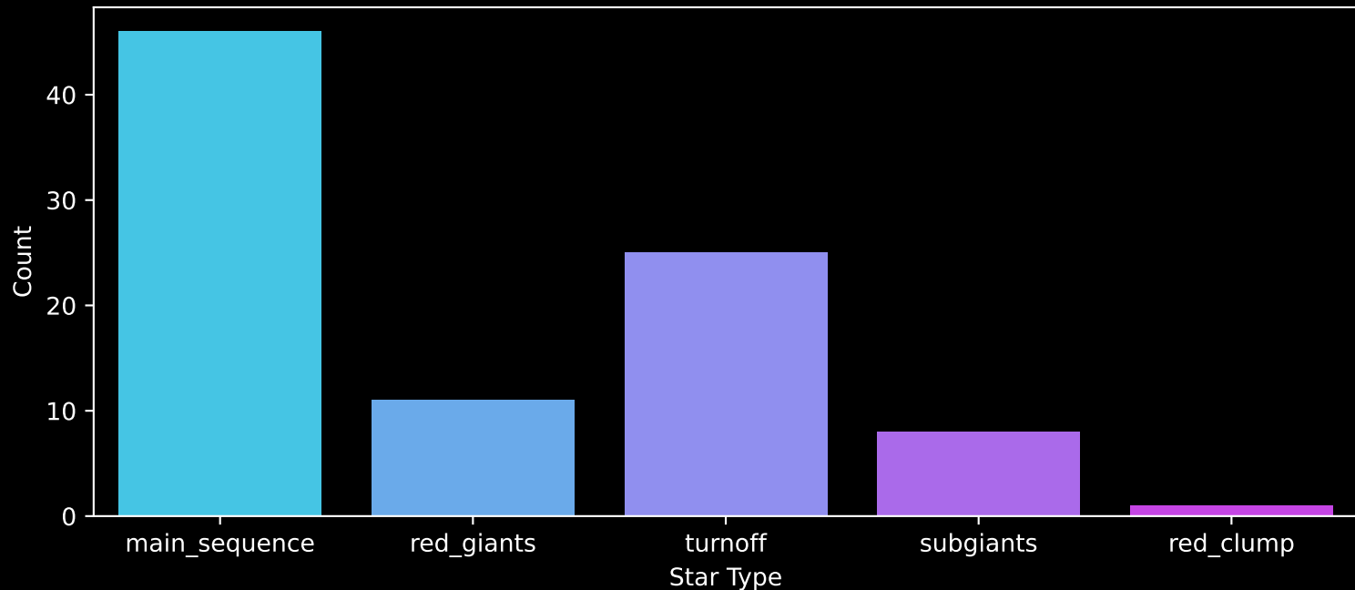
GALAH DR4 Field: [6683] Count plot of Star Type
