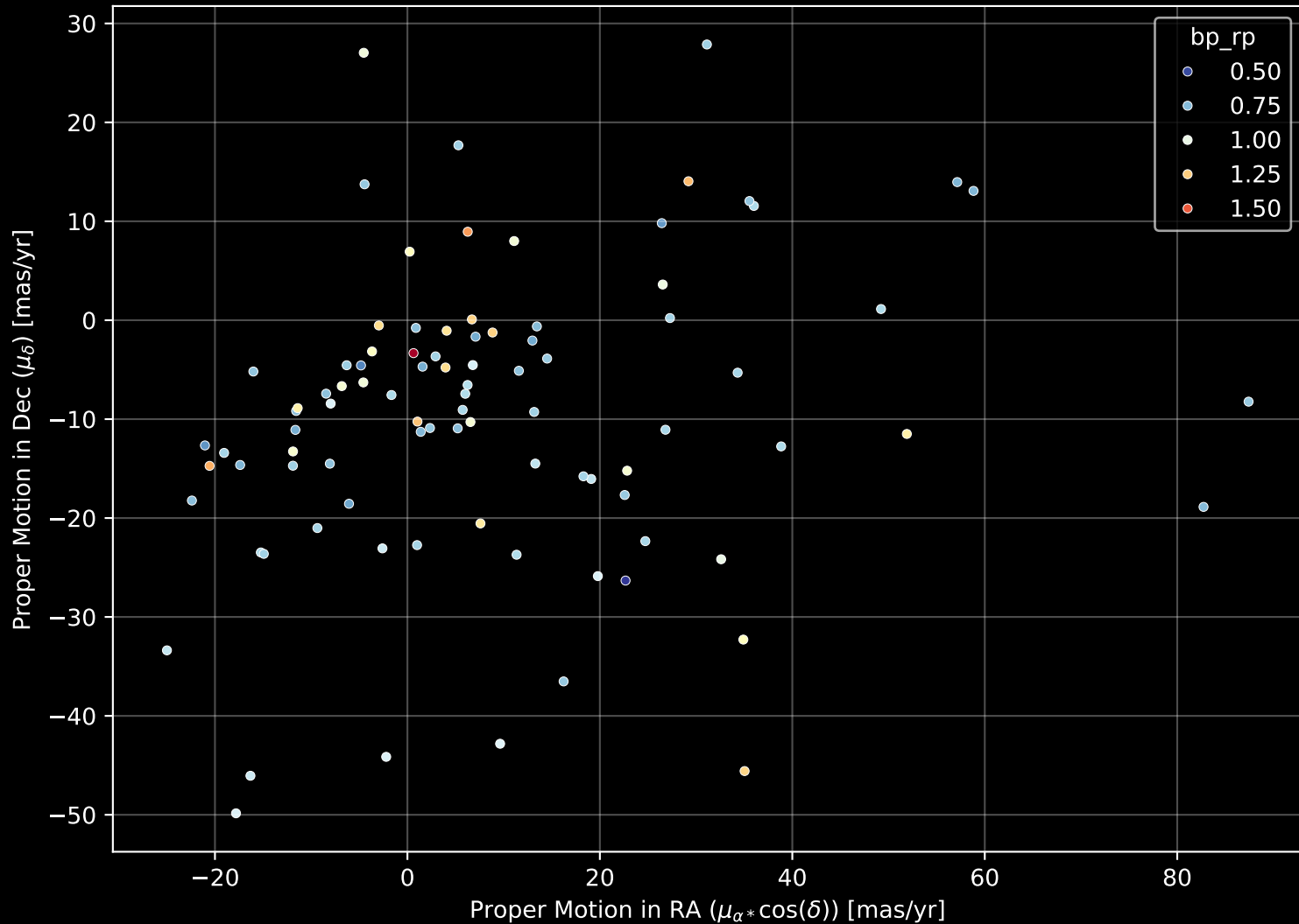
GALAH DR4 Field: [6683] Proper Motion Diagram (n= 91)
